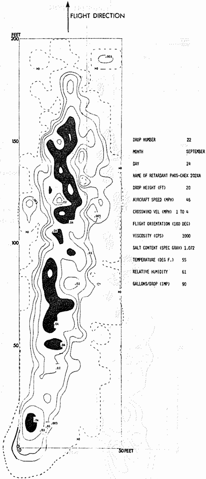
FIGURE 18. A GROUND DISTRIBUTION PATTERN FOR THE LODGEPOLE PINE STAND WITH THE SIMS BUCKET.
